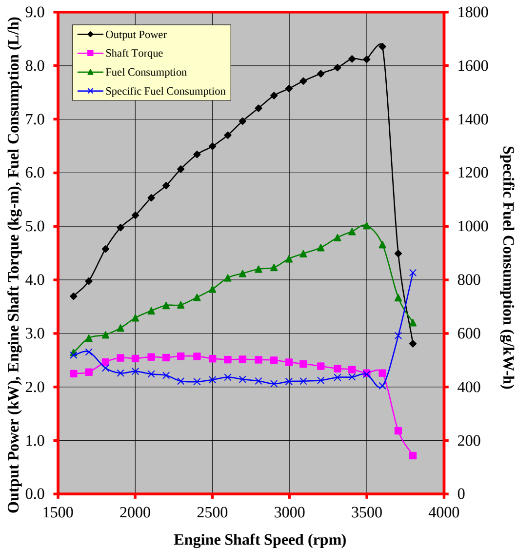
Figure 3. Performance characteristic curves of the KENBO KB18 2F gasoline engine
