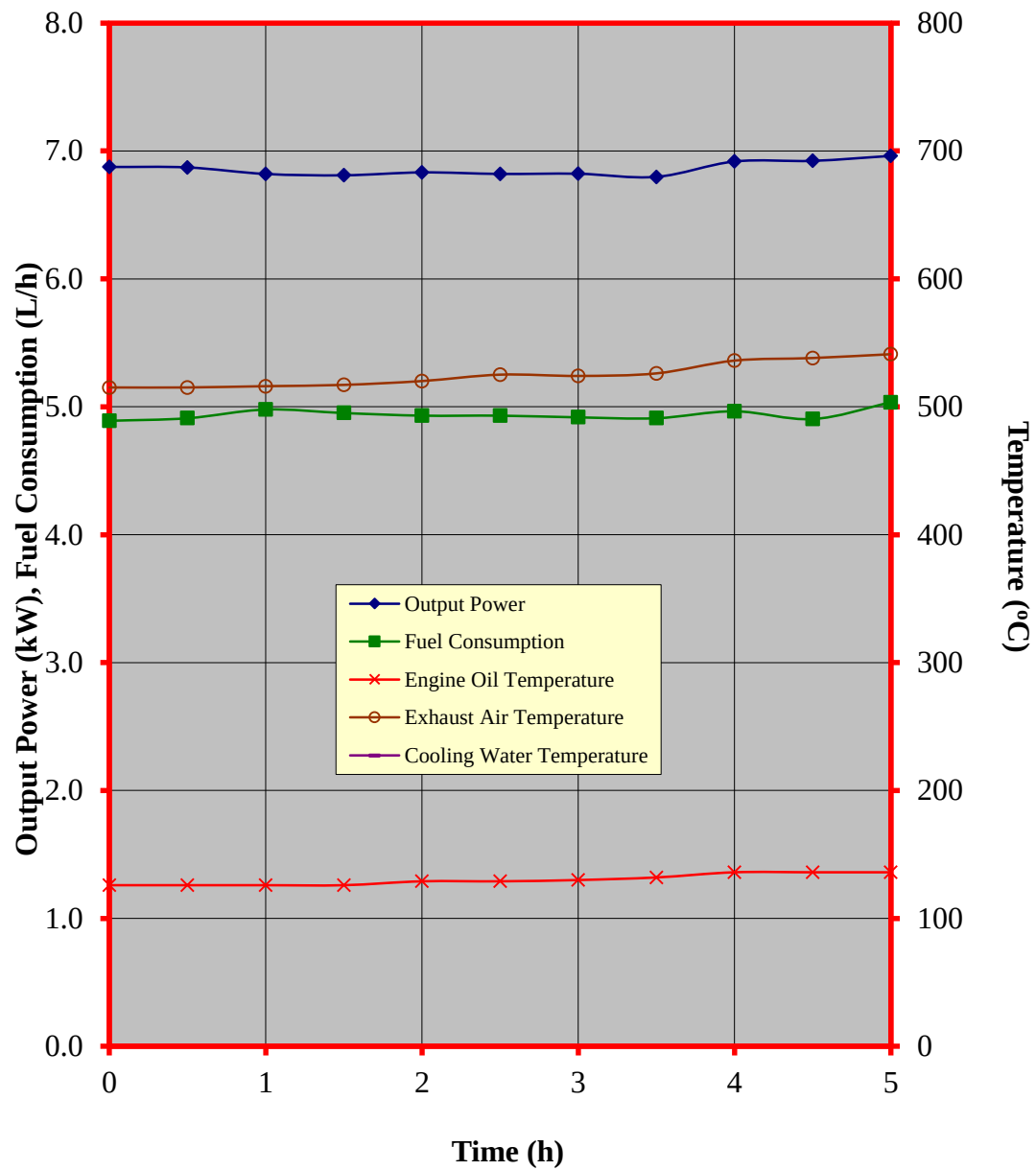
Figure 4. Performance characteristic curves during the continuous running test of the KENBO KB18 2F gasoline engine
